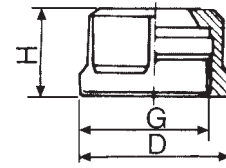
FIG.3 ER11,16,20UM
